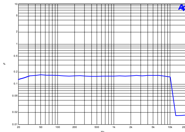
Figure 14. THD+N vs. Frequency, 1W
