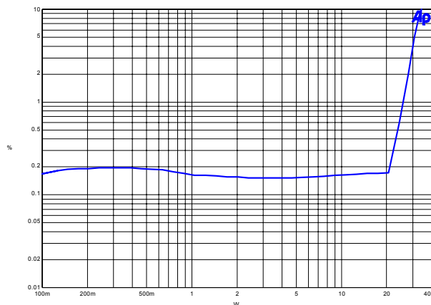
Figure 13. THD+N vs. Output Power @ 1kHz
