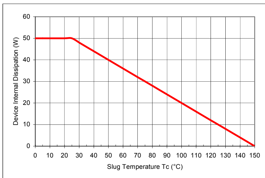
Figure 5 –Power Derating Curve (Typical)
