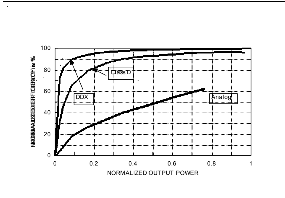
Figure 3 – Efficiency Comparison, Damped Ternary and Binary Modulation
