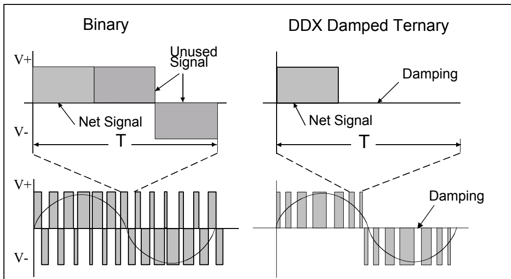
Figure 2 – Comparison of Binary and DDX Damped Ternary Modulation
