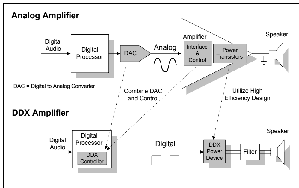
Figure 1 - DDX and Amplifier Architecture Comparison
